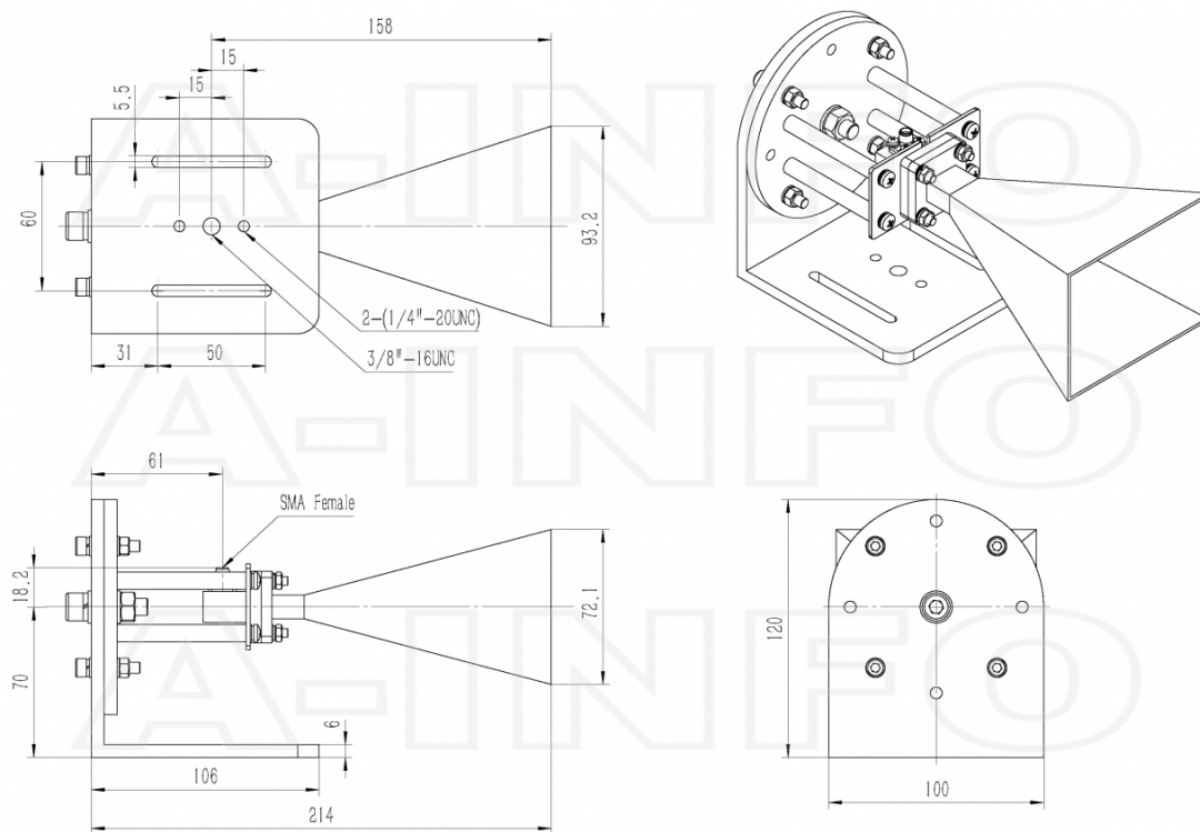
SMA-Female Output with L Type Mounting Bracket (Option, P/N: LB-62-10-C-MBL)
