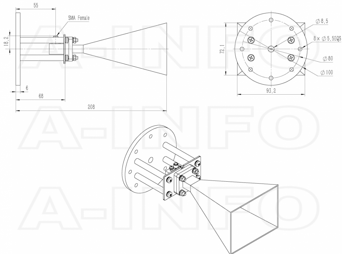
SMA-Female Output with Round Mounting Bracket (Option, P/N: LB-62-10-C-MB)
